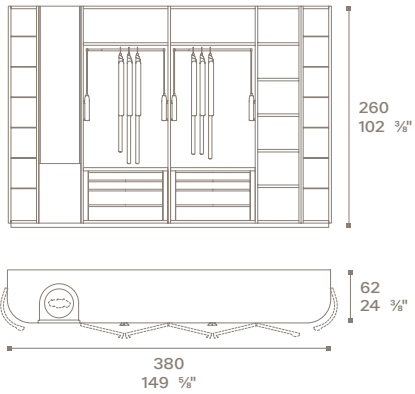
Wardrobe (doors open)
